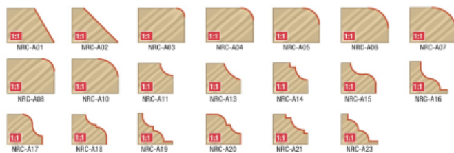
Body Type A (Edge Form Routing) Profiles
