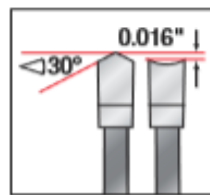
HOLLOW GROUND
