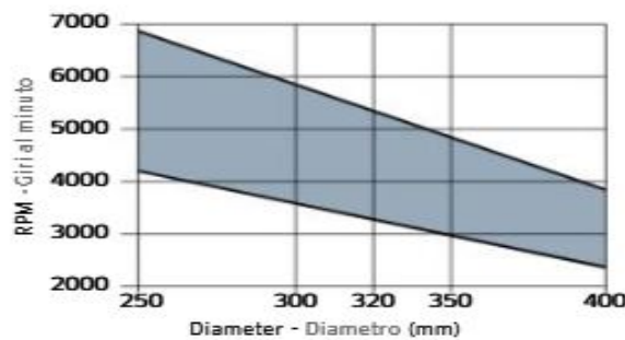
Minimum and maximum RPM based on the blade diameter.
