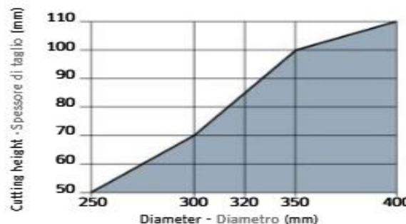
Maximum depth of cut based on the blade diameter.
