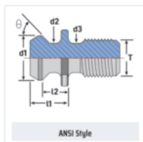
CAT Retention Knobs
