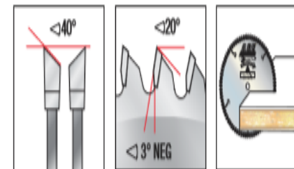
H-ATB GRIND HIGH OR ACUTE ANGLE ALTERNATE TOP BEVEL
