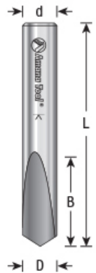
Drill Point 118°
