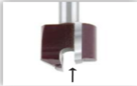
A proper mortising bit should have a large gullet between the two flutes which allows for greater chip clearance and removal.
